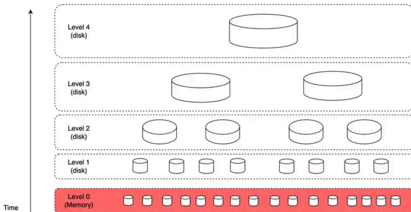
Figure 11 LSM tree
