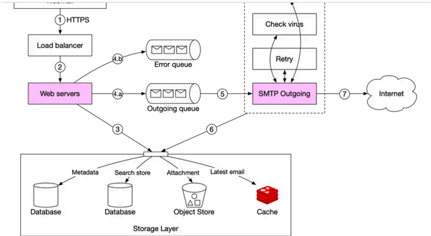
Figure 6 Email sending flow
